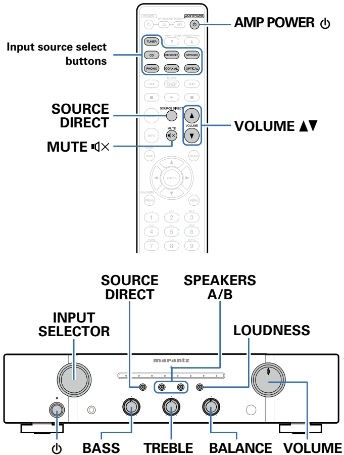
Front panel
